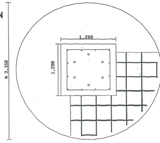
MAT CONSISTS OF 10 BY 10 BARS AT 328mm SPACING
